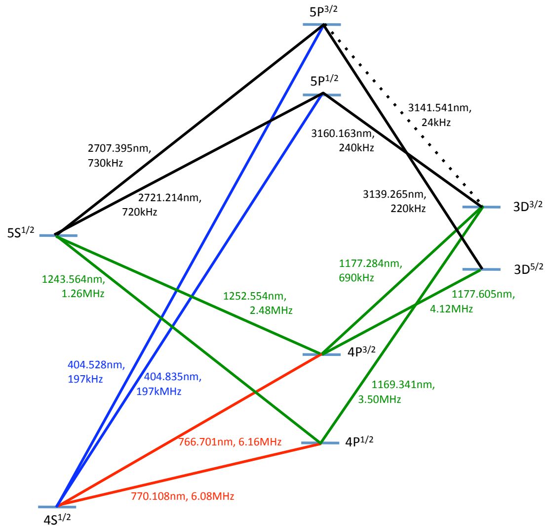
^{40}\text{K} transition diagram
